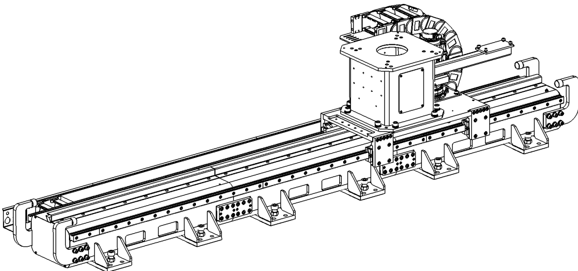
Linear track with robot pedestal
