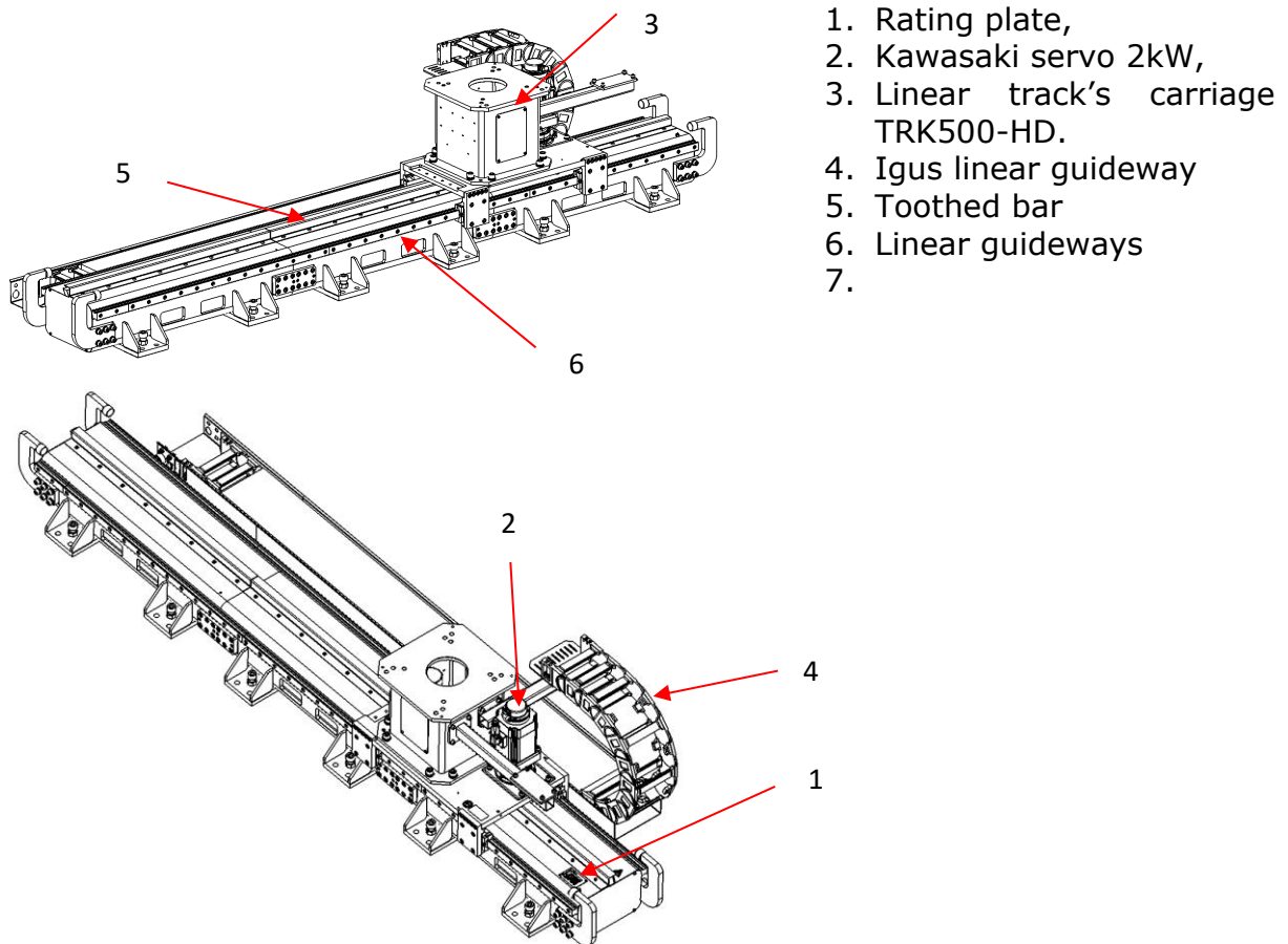
Fig. 2. Basic assembly of the basic module
